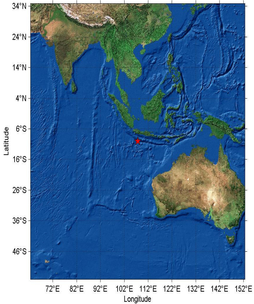
Epicenter Location Map (South of Java, Indonesia)
