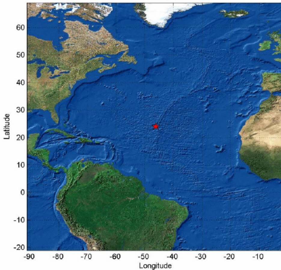
Epicenter Location (Northern Mid Atlantic Ridge 6.6 Moderate)
