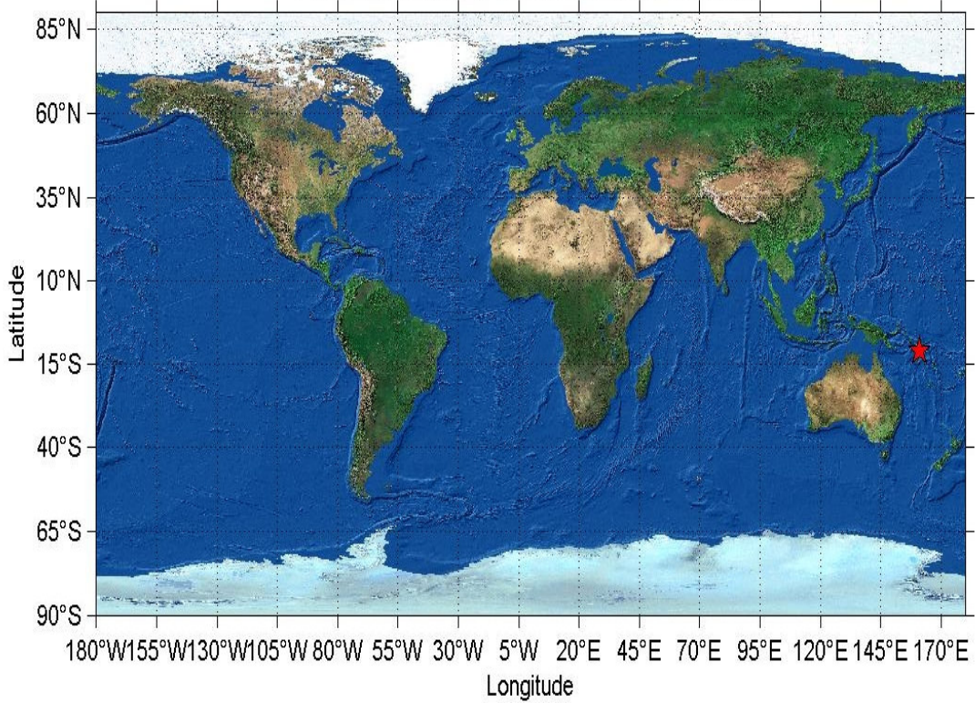
Epicenter Location (Solomon Islands 6.8 Moderate)
