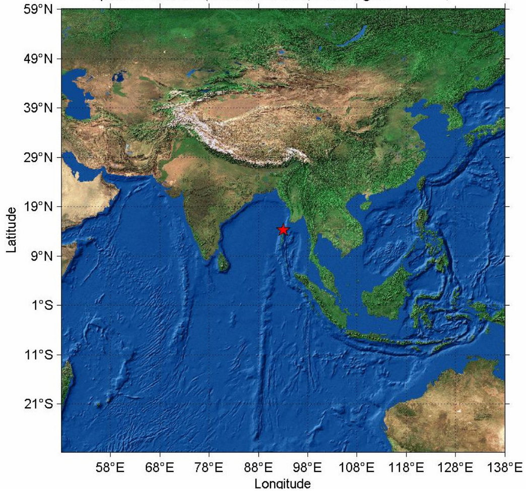
Epicenter Location (Andaman Islands, India Region 7.6 Great )
