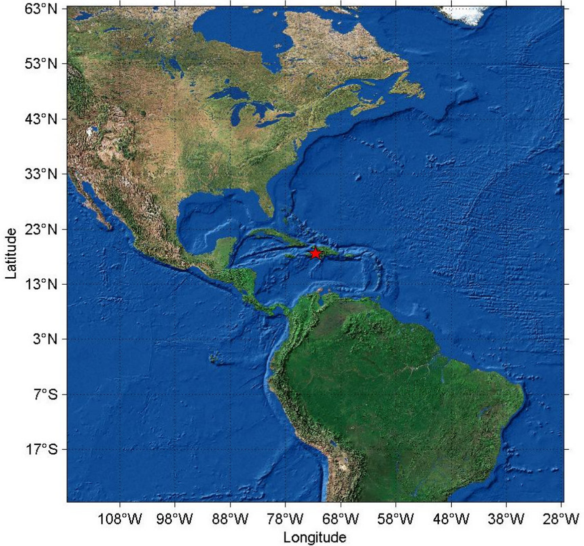
Epicenter Location (Haiti Region 6.5 Moderate)
