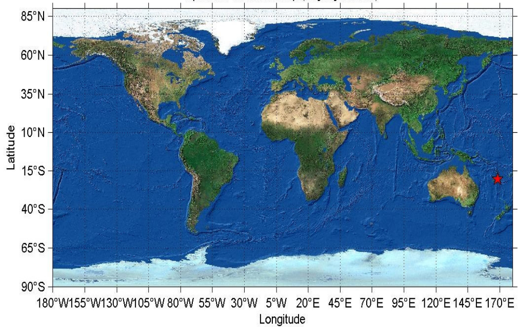
Epicenter Location Map (Loyalty Islands)
