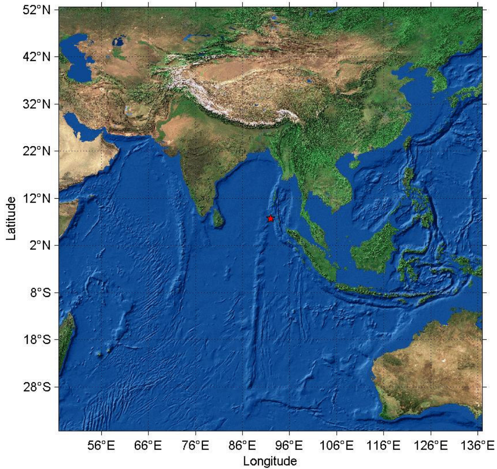
Epicenter Location (Andaman Nicobar Islands Region 7.5 M Great)
