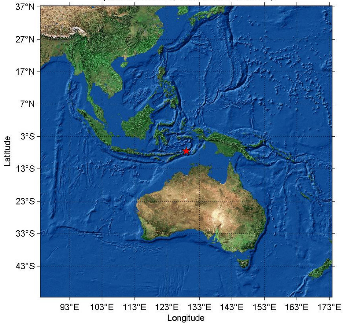
Epicenter Location (Banda Sea 6.7 Moderate)
