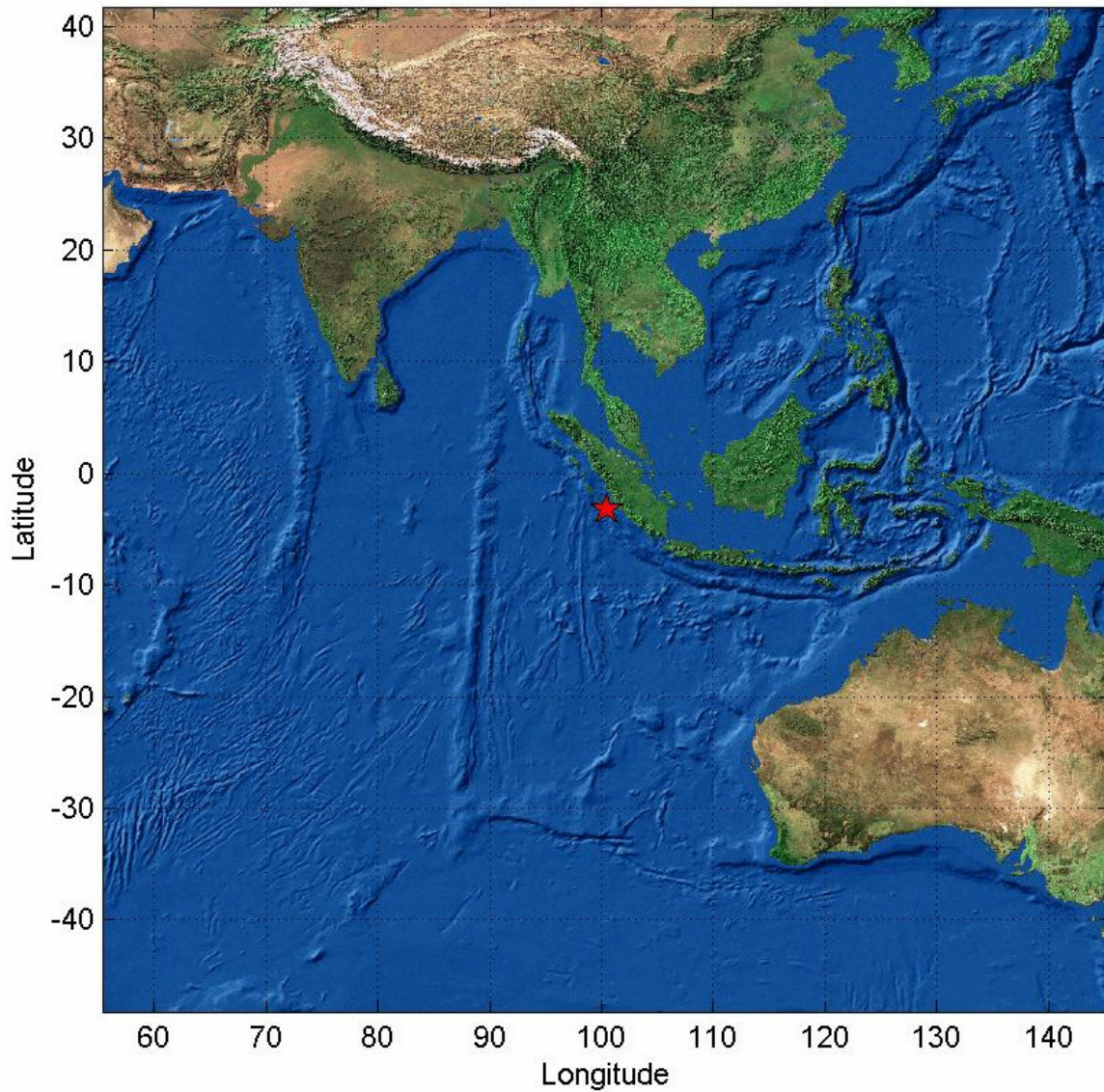
Epicenter Location (Southern Sumatra, Indonesia 6.0 Moderate)
