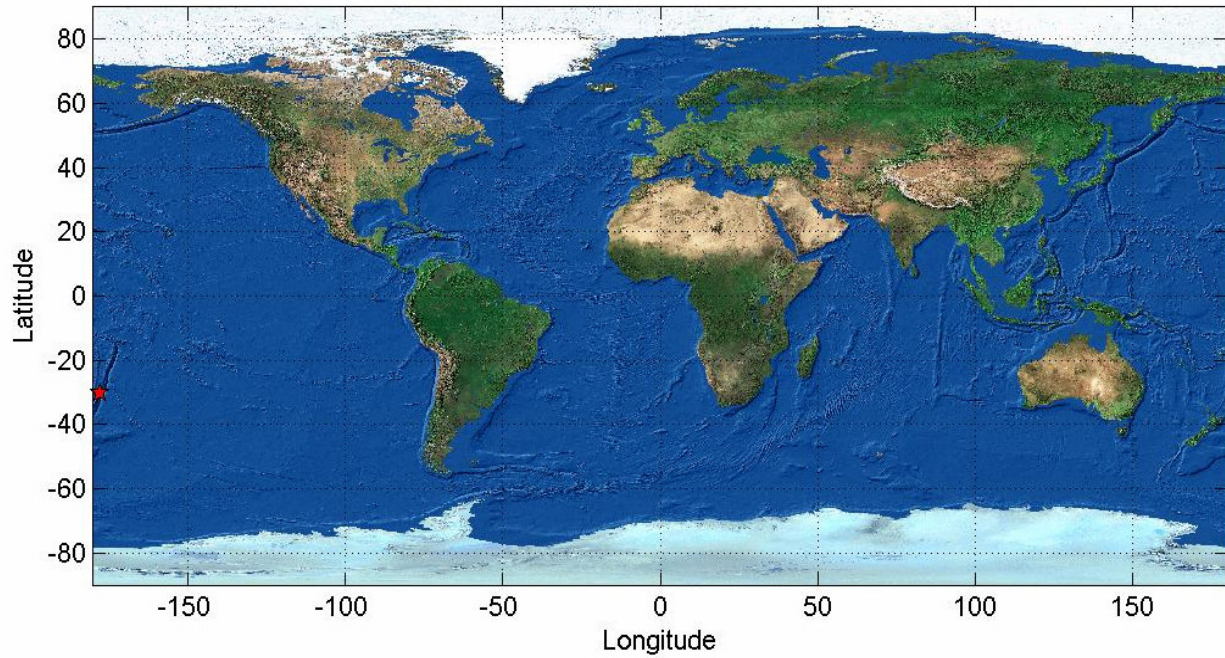
Epicenter Location (Kermadec Islands, New Zealand 7.1 Mw Great)
