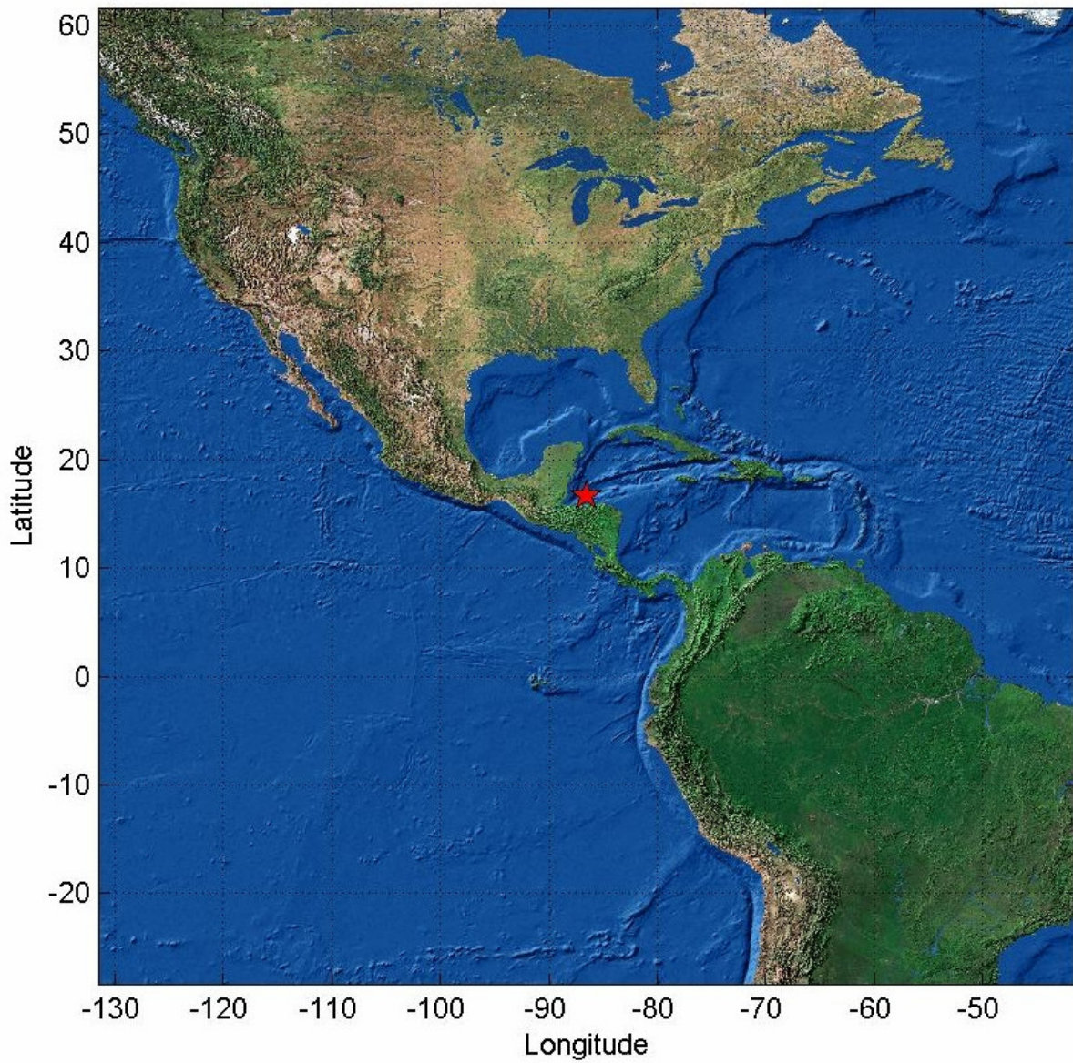
Epicenter Location (North of Honduras 7.1 Great)
