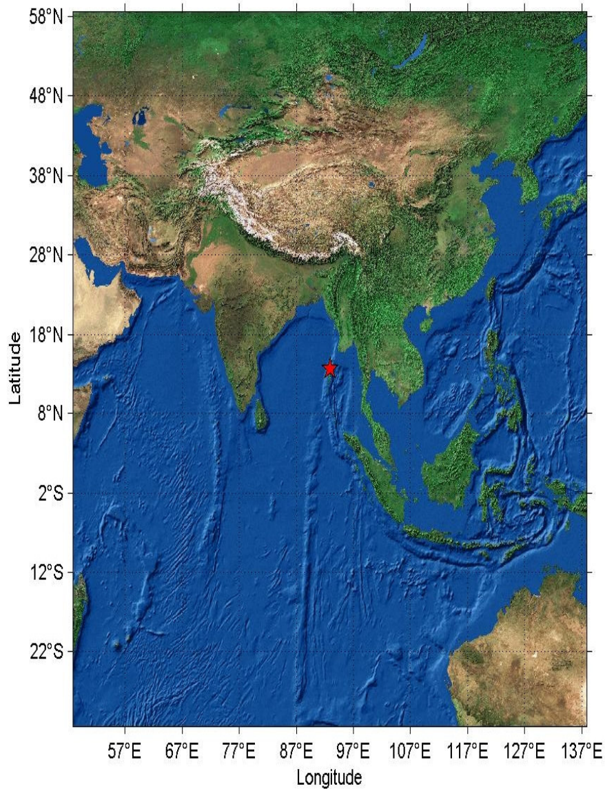
Epicenter Location (Andaman Islands, India Region 7.0 Great)
